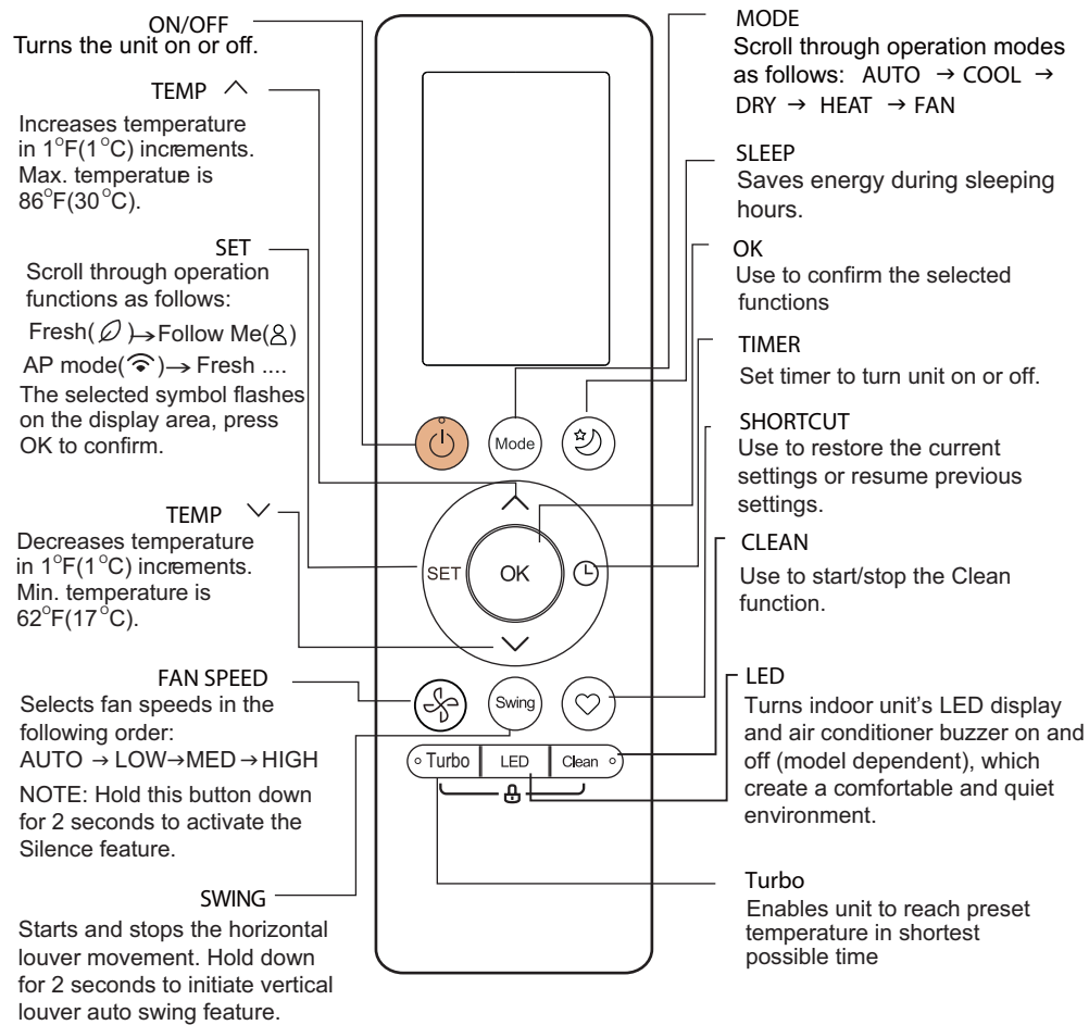
Fig. 5 — Remote Controller
