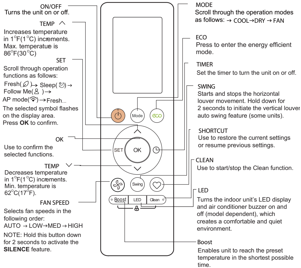
Fig. 7 — Remote Controller
