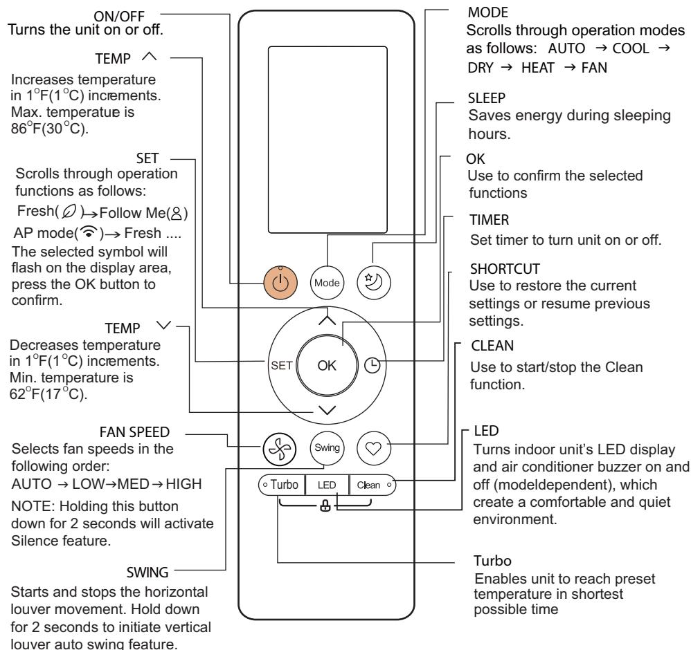
Fig. 3 — Wireless Remote Controller Functions
