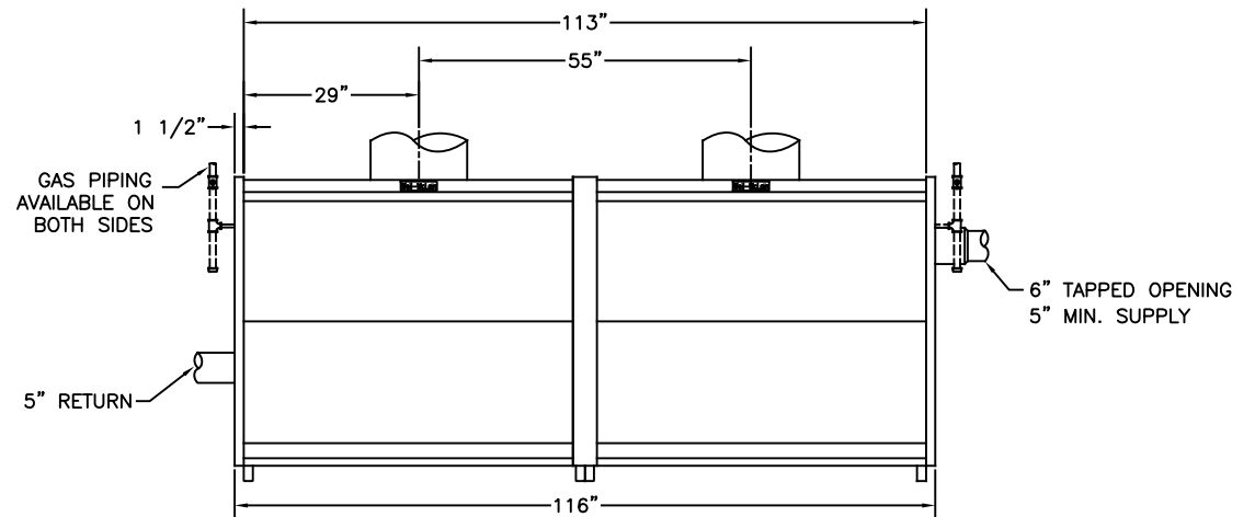
FRONT
